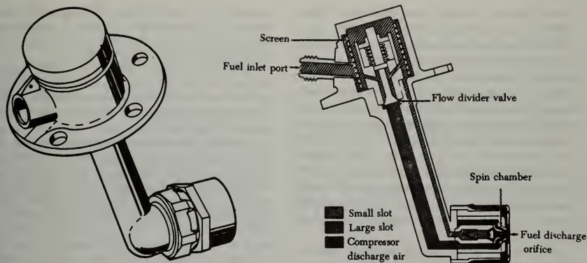
FIGURE 3-59. Duplex fuel nozzle.
